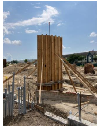
Amphitheater Pedestal Formwork
