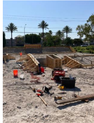
Skatepark Formwork
