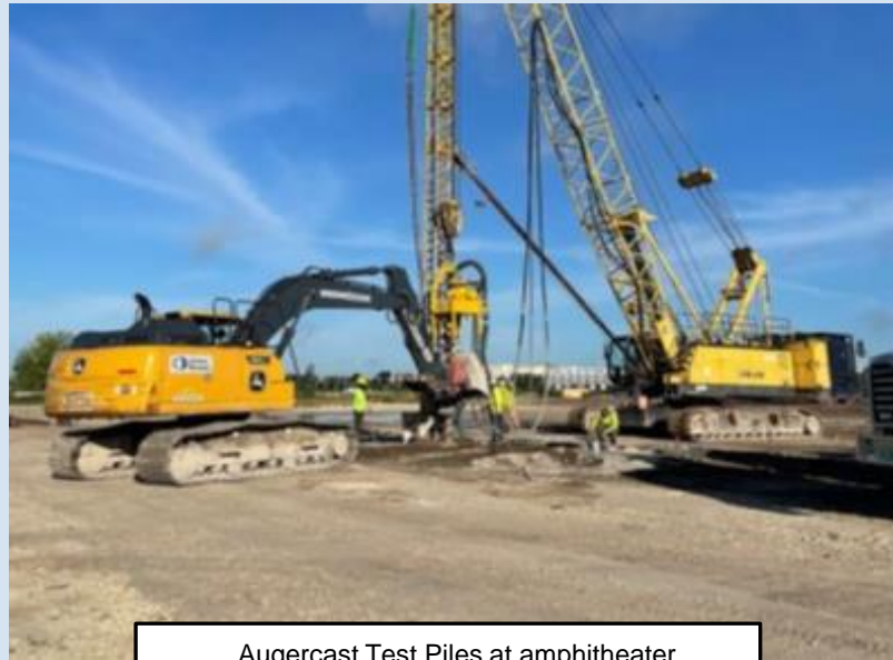
Augercast Test Piles at amphitheater
